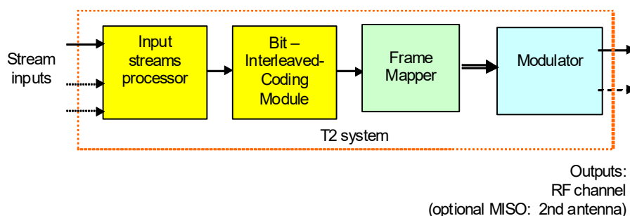
Figure 4.19: High level T2 block diagram
