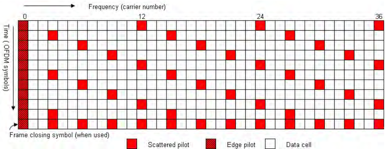
Figure 2.6: Pilot pattern 1 - SISO (from [EN 302 755 V1.3.1])
