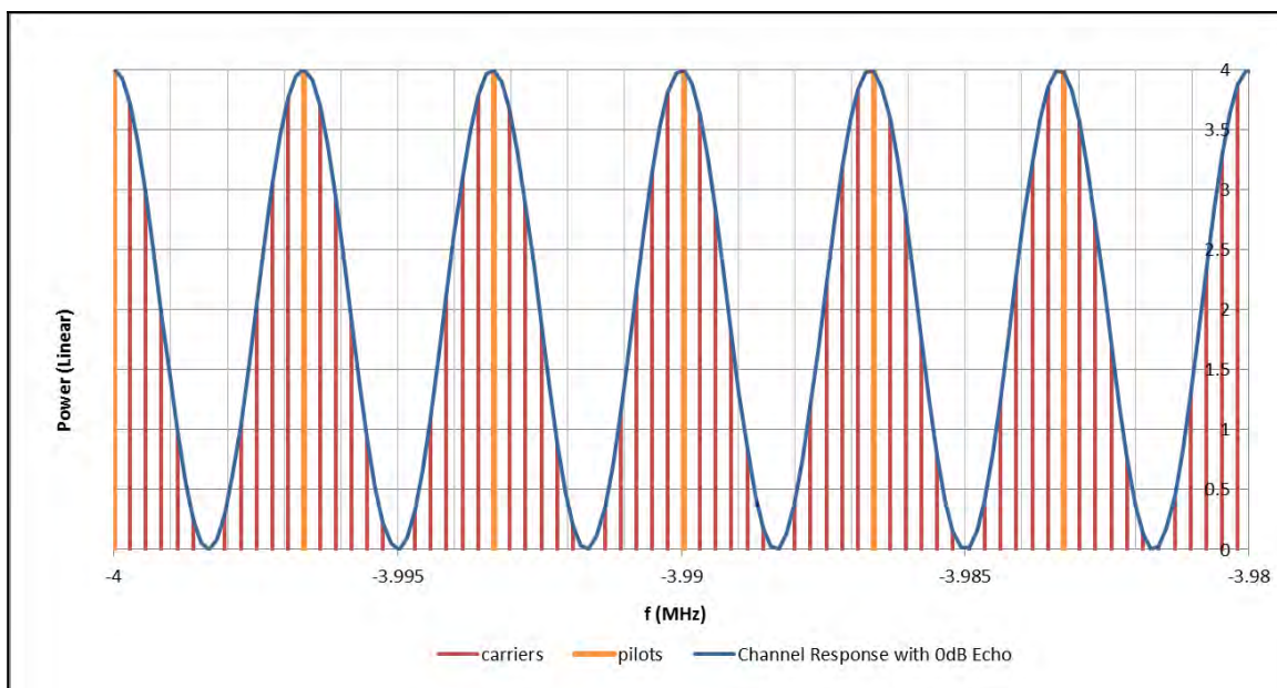
Figure A6.5: DTT passband in a perfect channel with 0 dB echo at 300 μs delay - linear amplitude
