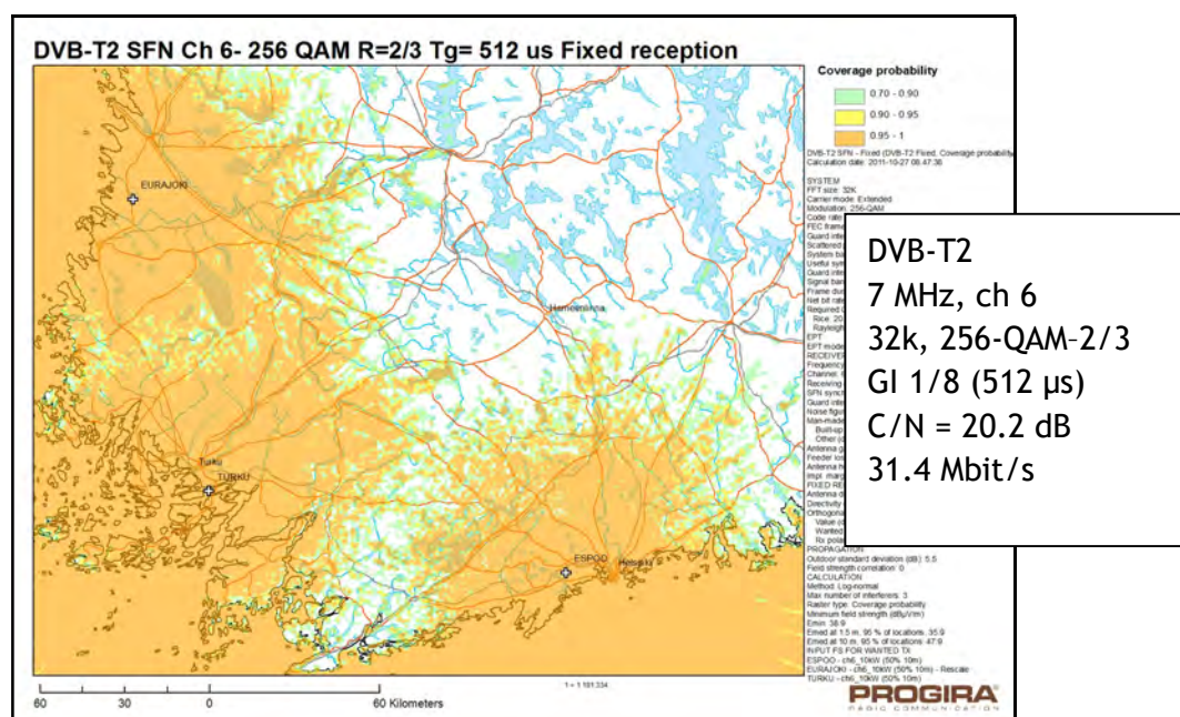
Figure 4.2: Rooftop Reception, SFN, Large Area, VHF, DVB-T2 in Finland
