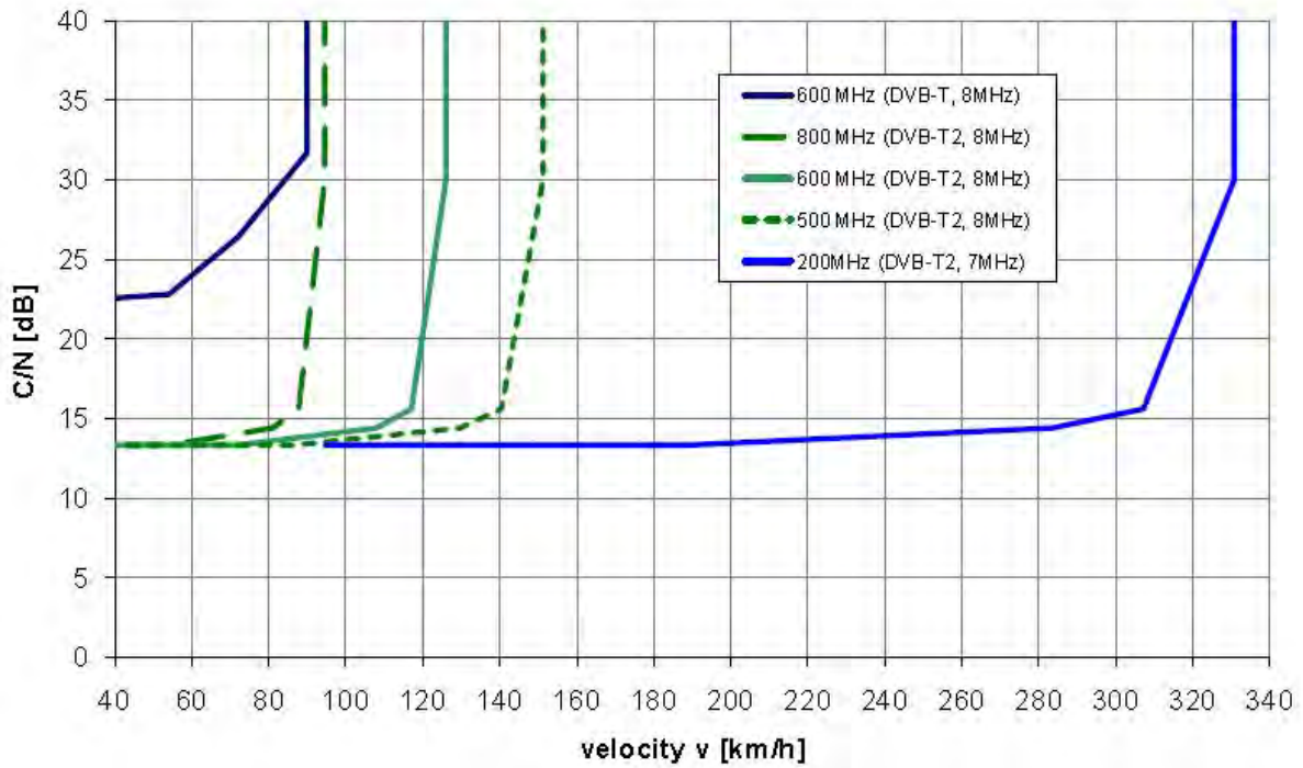
Figure 2.10: Required C/N for DVB-T and DVB-T2 as a function of the velocity of the mobile receiver, 8k FFT (from [AFM2010])
