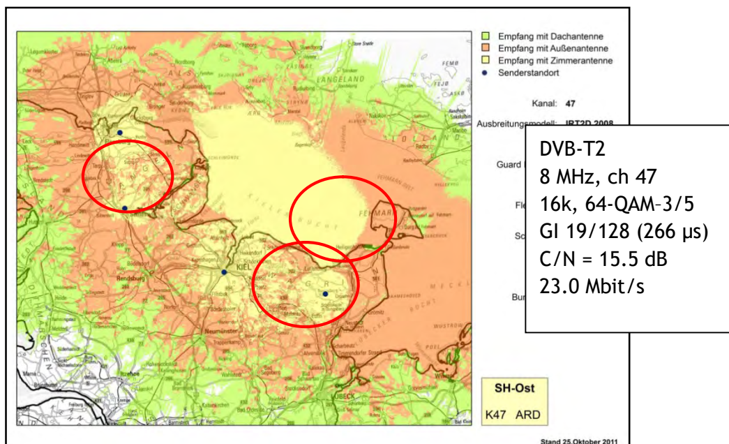
Figure 4.6: Portable Reception, SFN, Medium Area, UHF, DVB-T2 in the northern part of Germany
