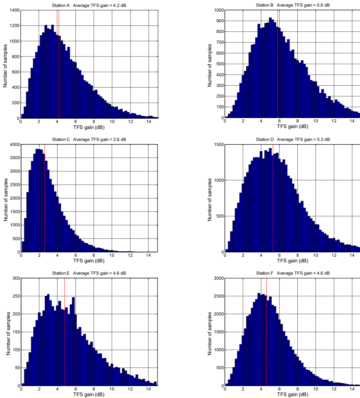
Figure 4.18: Measured distribution of TFS gain
