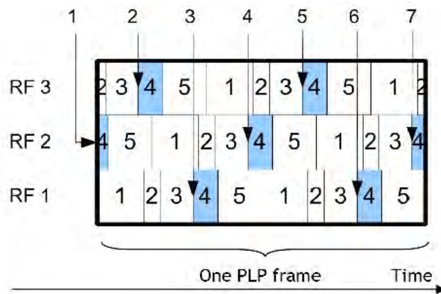
Figure 4.16: Example, TFS over three frequencies
