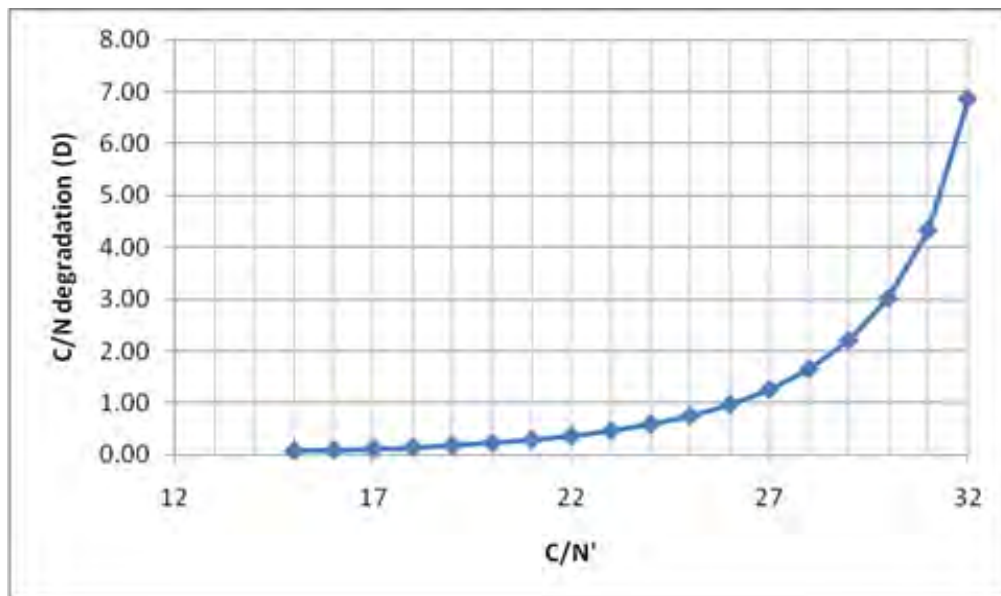
Figure 2.2: Factor D, C/N degradation (dB) for a back-stop noise level of -33 dBc
