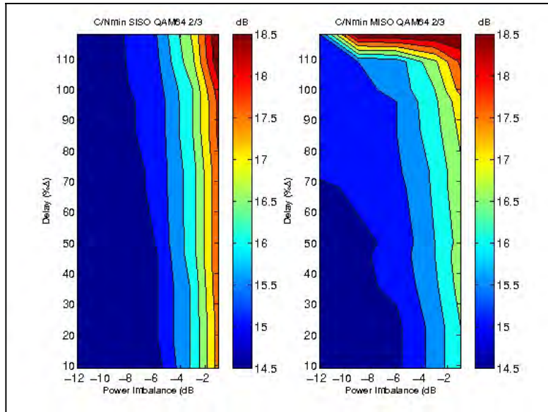
Figure 4.15: Required C/N as a function of the power imbalance and the time delay of the two MISO signals and the same signal configuration when operated in SISO mode for the SDR receiver and DVB-T2 mode 32k 64-QAM 2/3 GI 1/32 (from [Mo2013])
