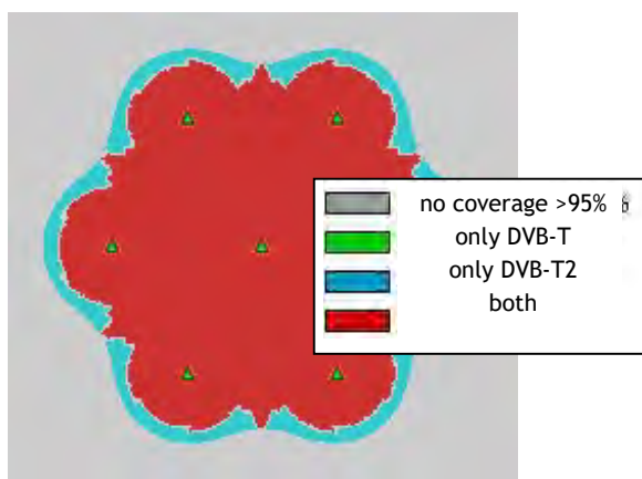
Figure 4.9: Comparison of the coverage areas for the 8k and the 32k FFT mode
