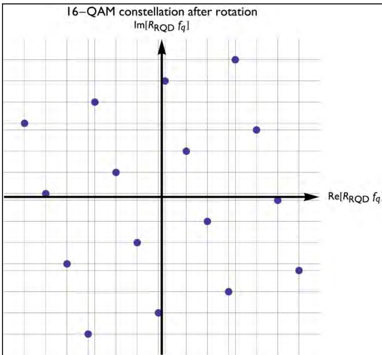
Figure 2.4: Rotated constellation diagram for 16-QAM modulation (from [TS 102 831])
