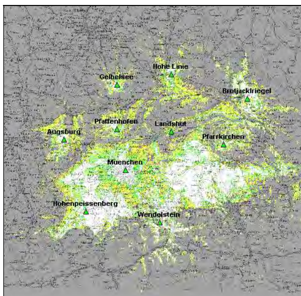
Figure 4.8: Portable Reception, Hypothetical SFN, Large Area, UHF, DVB-T in Bavaria
