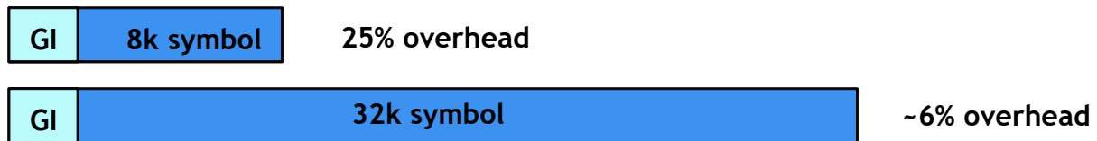
Figure 2.12: Guard interval overhead reduction with larger FFT size
