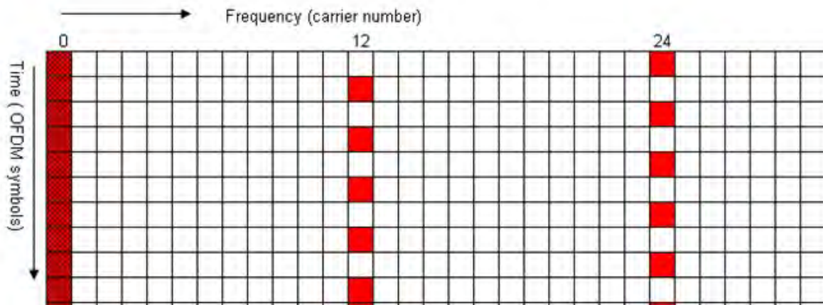
Figure A6.3: Scattered pilot pattern PP4 (SISO)
