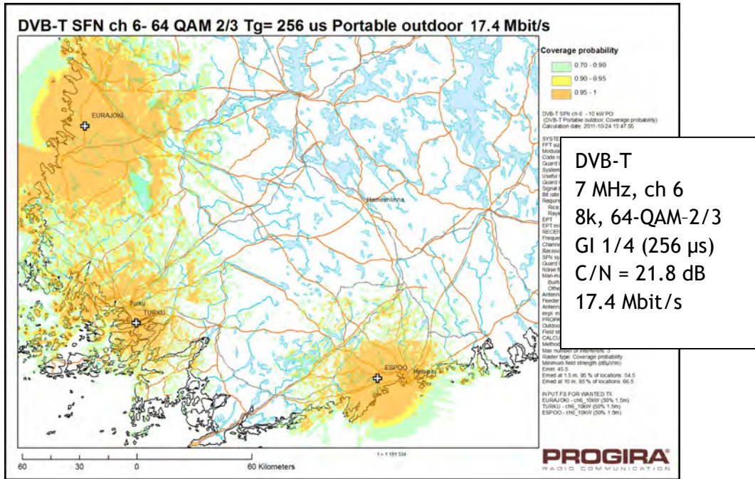
Figure 4.3: Portable Reception, SFN, Large Area, VHF, DVB-T in Finland
