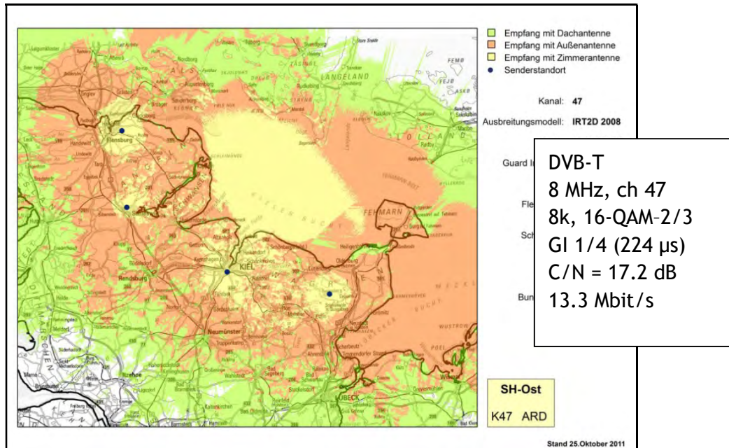
Figure 4.5: Portable Reception, SFN, Medium Area, UHF, DVB-T in the northern part of Germany
