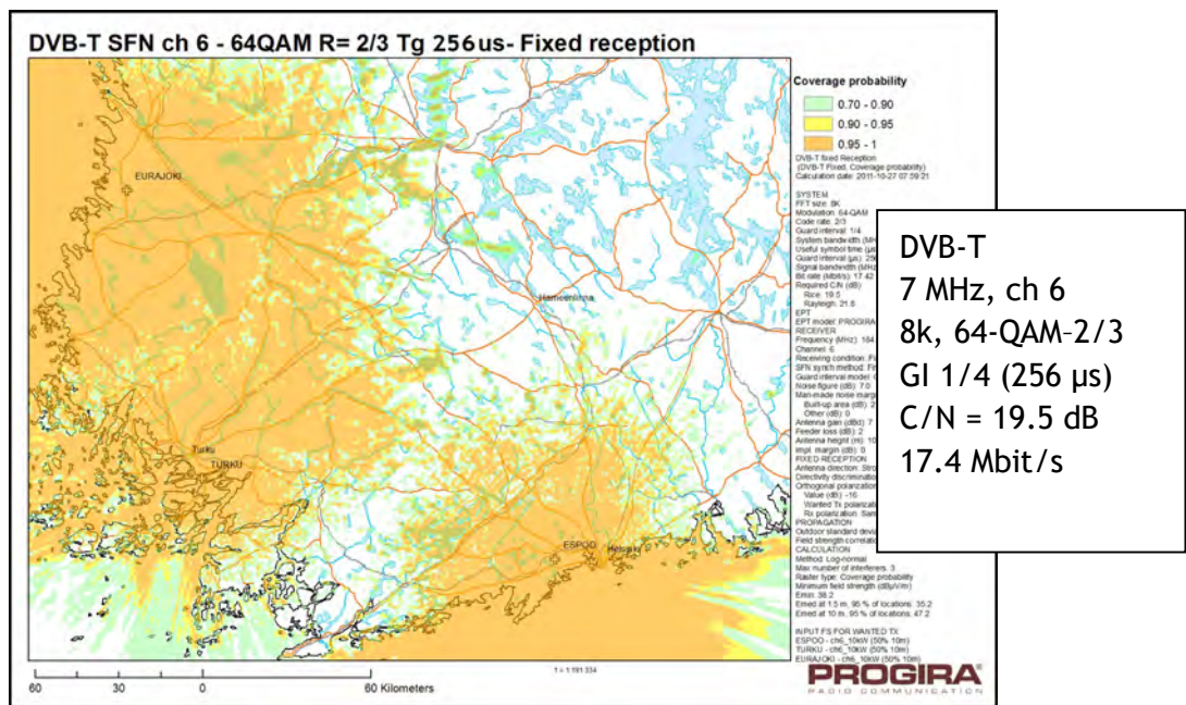
Figure 4.1: Rooftop Reception, SFN, Large Area, VHF, DVB-T in Finland
