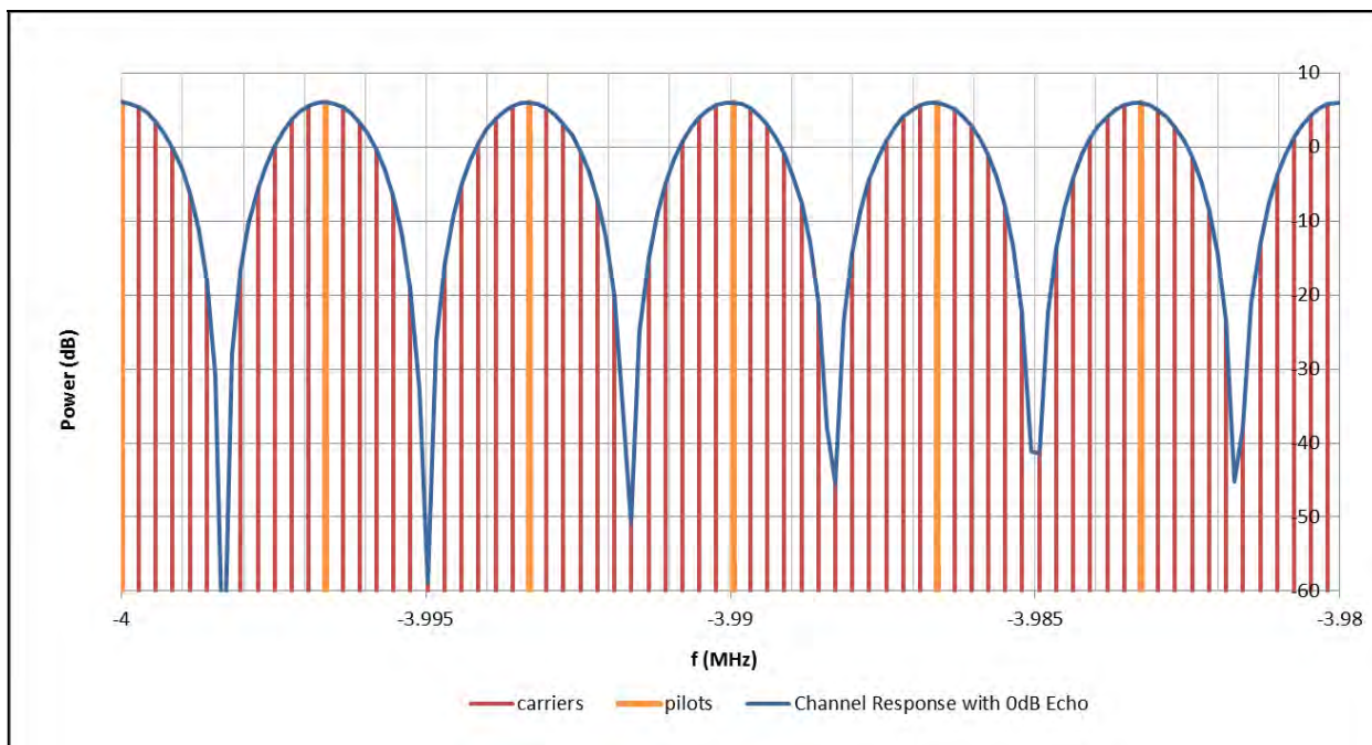
Figure A6.4: DTT passband in a perfect channel with 0 dB echo at 300 μs delay
