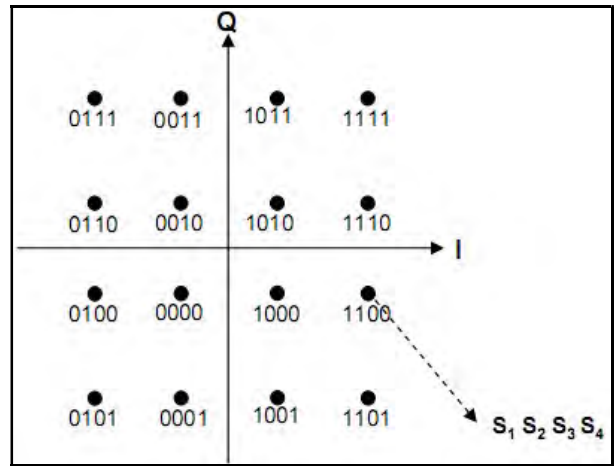
Figure 2.3: Constellation diagram for 16-QAM modulation (Figure taken from [ND2008])
