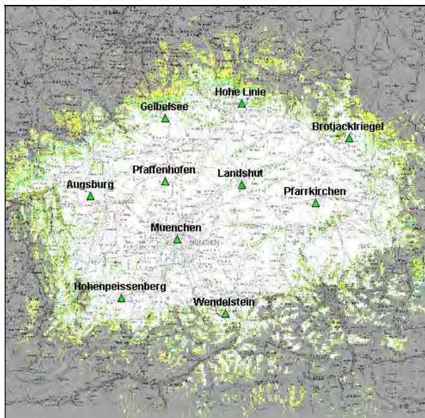
Figure 4.7: Portable Reception, SFN, Large Area, UHF, DVB-T2 in Bavaria
