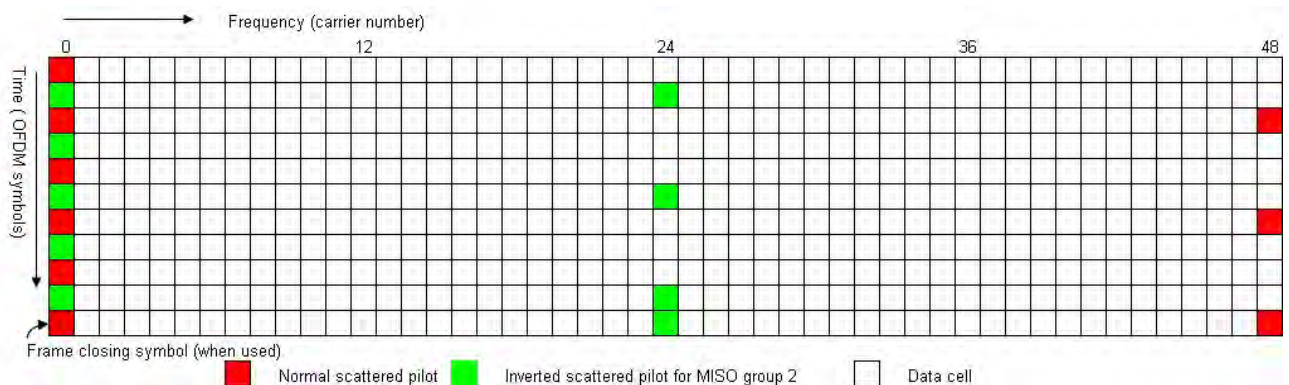
Figure 2.9: Pilot Pattern 7 - MISO (from [EN 302 755 V1.3.1])
