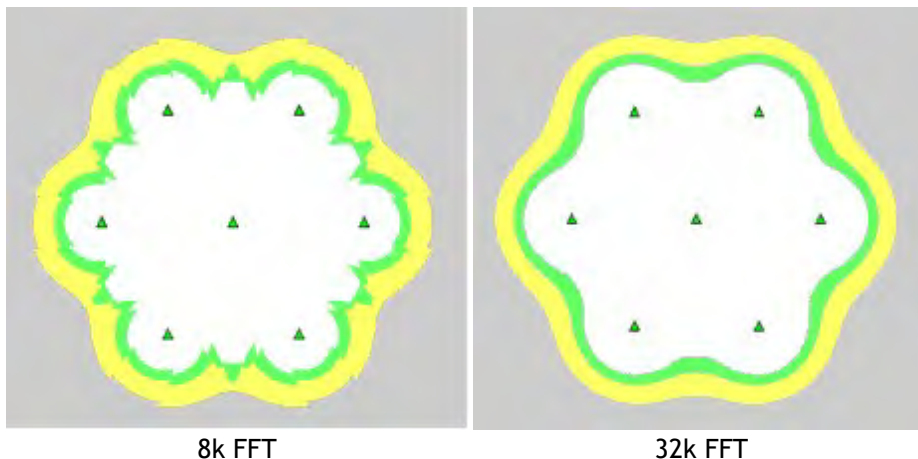
Figure 4.9: Comparison of the coverage areas for the 8k and the 32k FFT mode
